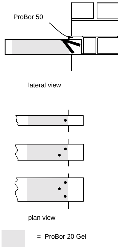
Figure 11: Embedded joist ends
