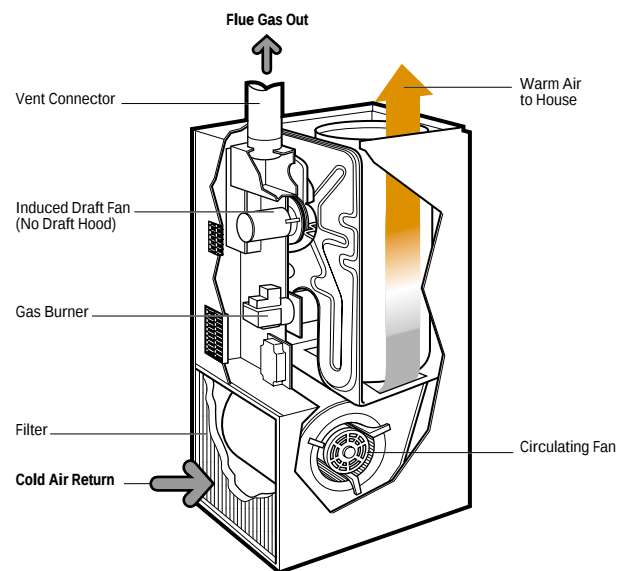
Figure 8 Standard-efficiency gas furnace with induced draft fan
