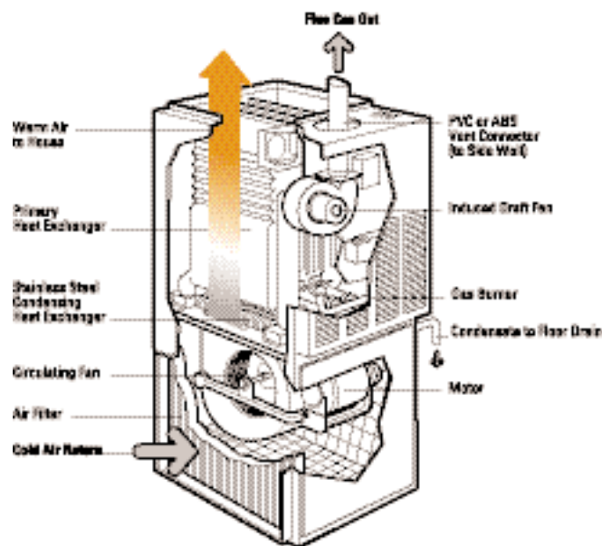
Figure 10 High-efficiency condensing gas furnace
