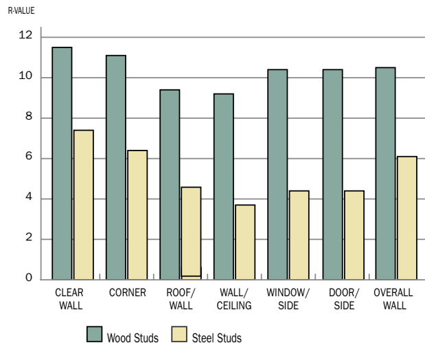
FIGURE 1 – Thermal Resistances of Wall Components with R-12 Insulation
